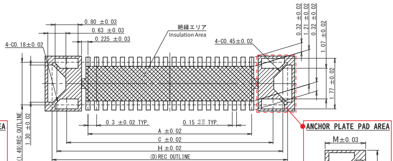
MOUNTING LAYOUT
