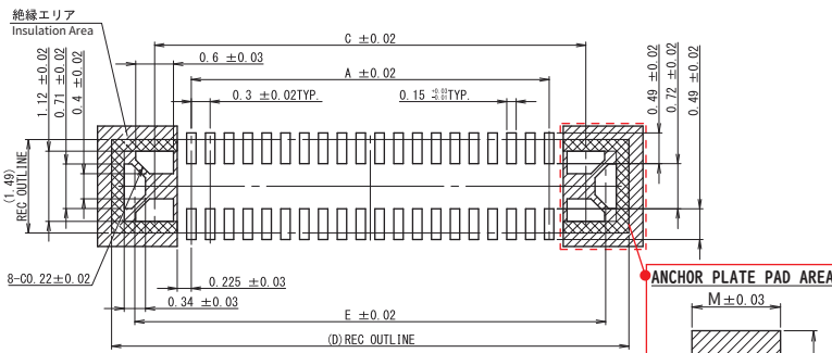
MOUNTING LAYOUT
