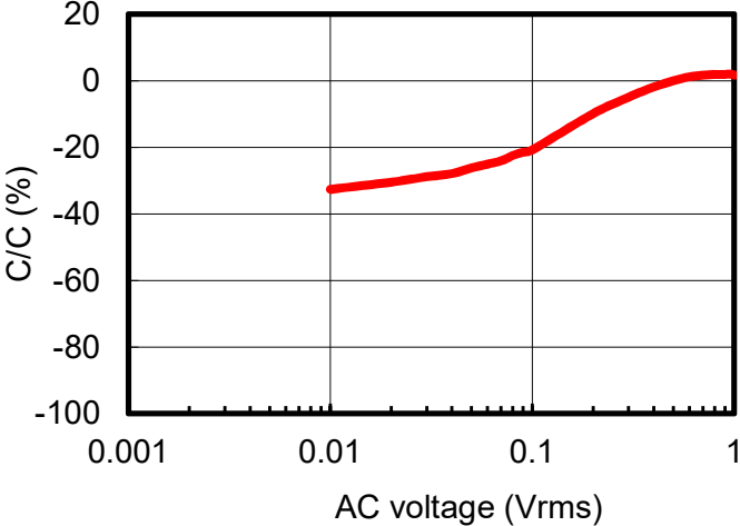
AC Voltage
