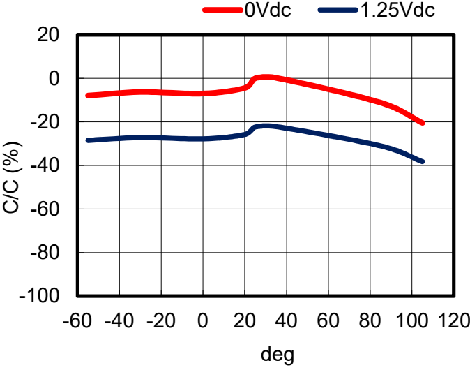
Temperature Characteristics
