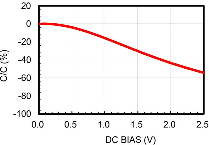
DC Bias
