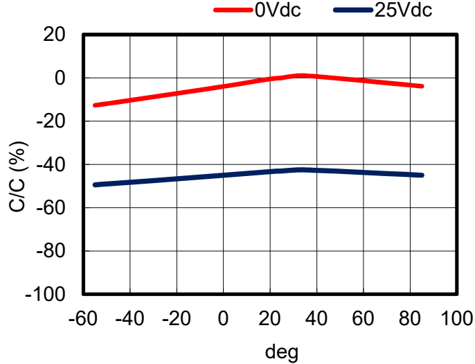
Temperature Characteristics
