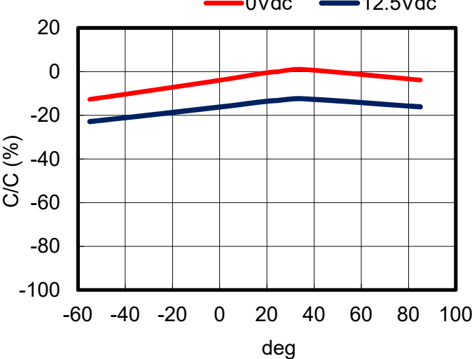
Temperature Characteristics
