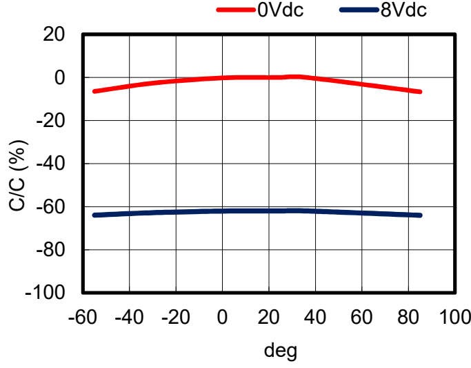
Temperature Characteristics
