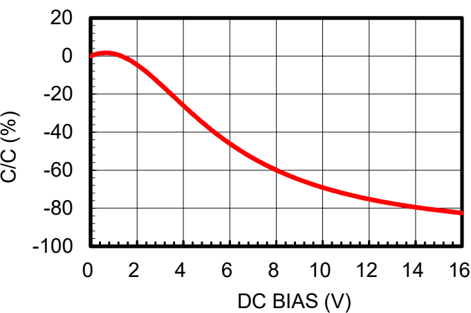
DC Bias
