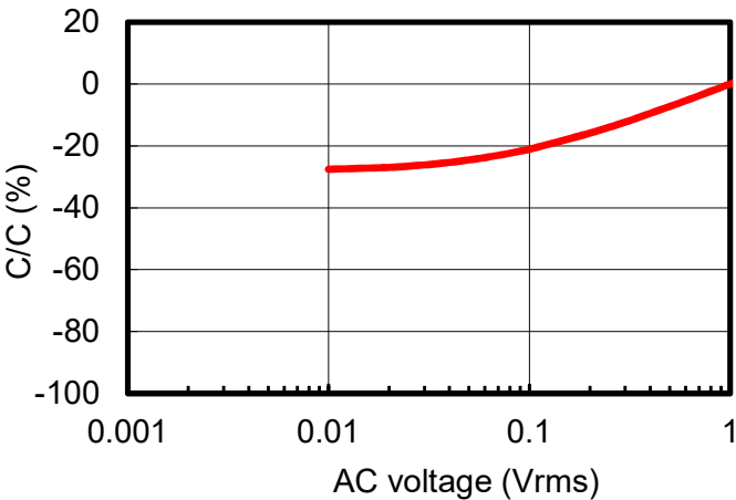
AC Voltage
