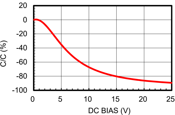
DC Bias
