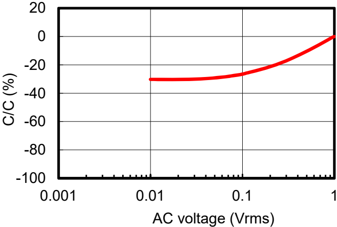
AC Voltage
