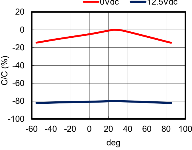
Temperature Characteristics
