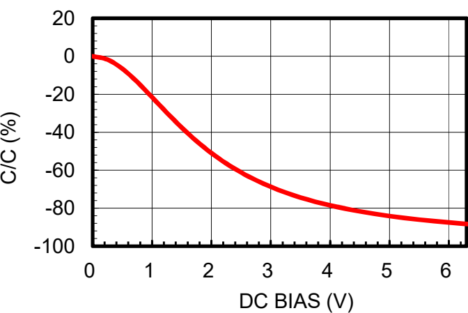
DC Bias
