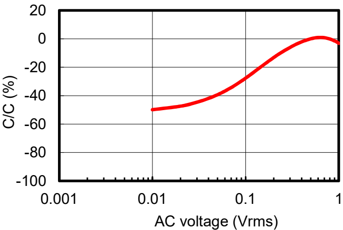
AC Voltage
