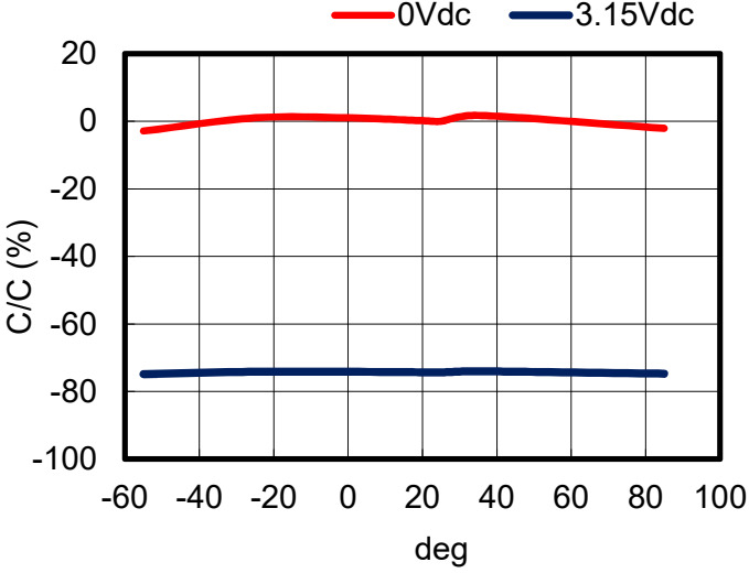
Temperature Characteristics
