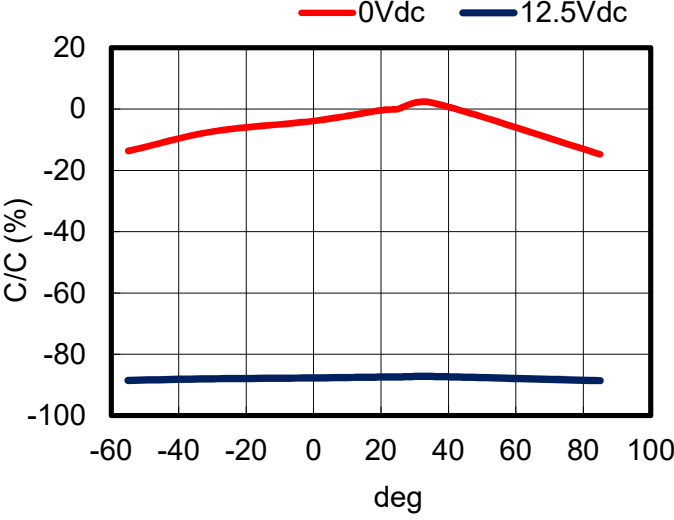
Temperature Characteristics
