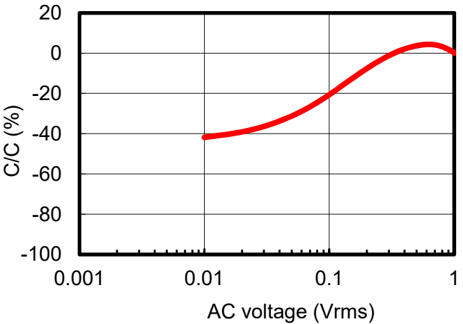
AC Voltage
