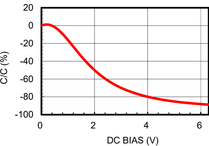
DC Bias
