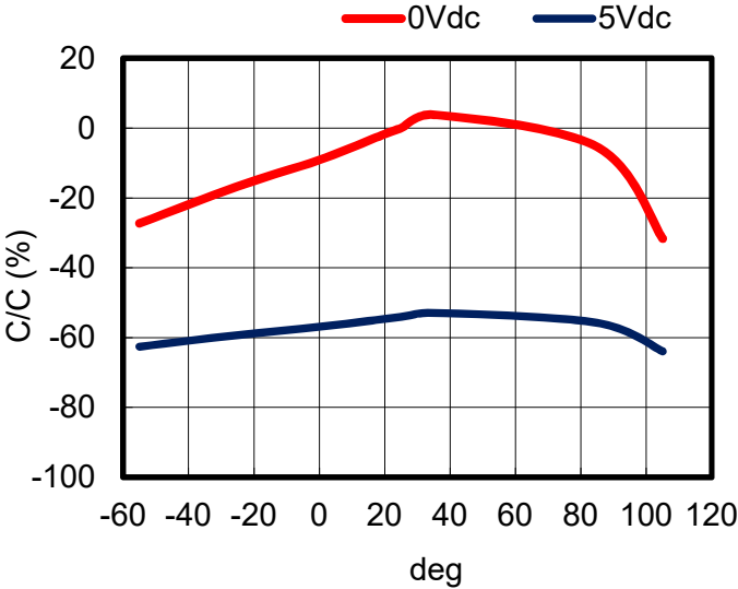
Temperature Characteristics
