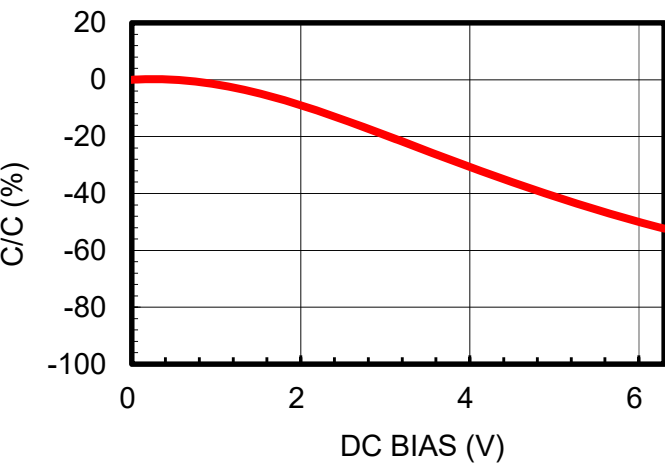
DC Bias
