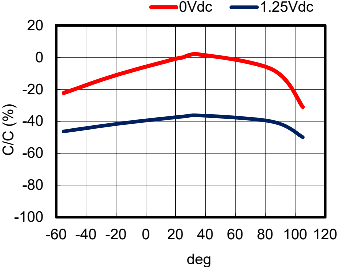
Temperature Characteristics
