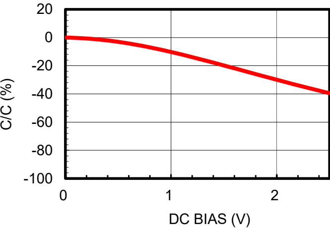
DC Bias
