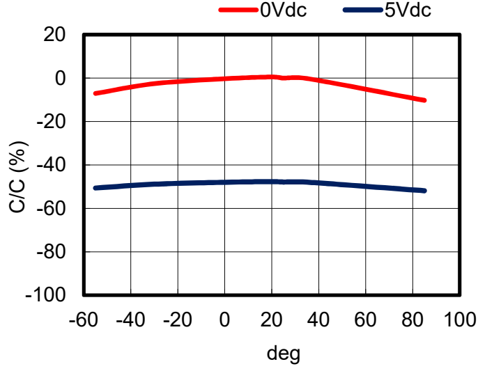
Temperature Characteristics
