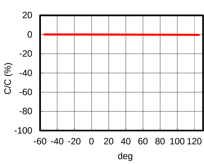
Temperature Characteristics
